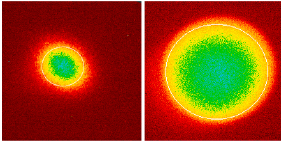
Fig. 9. (Left) MCP/phosphor image of 2.75 \times 10^4 antiprotons with a radius of approximately 2 mm. (Right) MCP/phosphor image of 5.6 \times 10^6 electrons with a radius of approximately 3.7 mm [69]. These plasma images were taken after the application of a rotating wall. The magnification factor due to the reduction of the magnetic field between the Catching Trap and the MCP is 8.3 (see Eq. (5) in Section 3.7), resulting in calculated radii of around 0.25 mm (antiprotons) and 0.45 mm (electrons) in the trap. White circles indicate the approximate plasma size and location as determined by a fit function.
