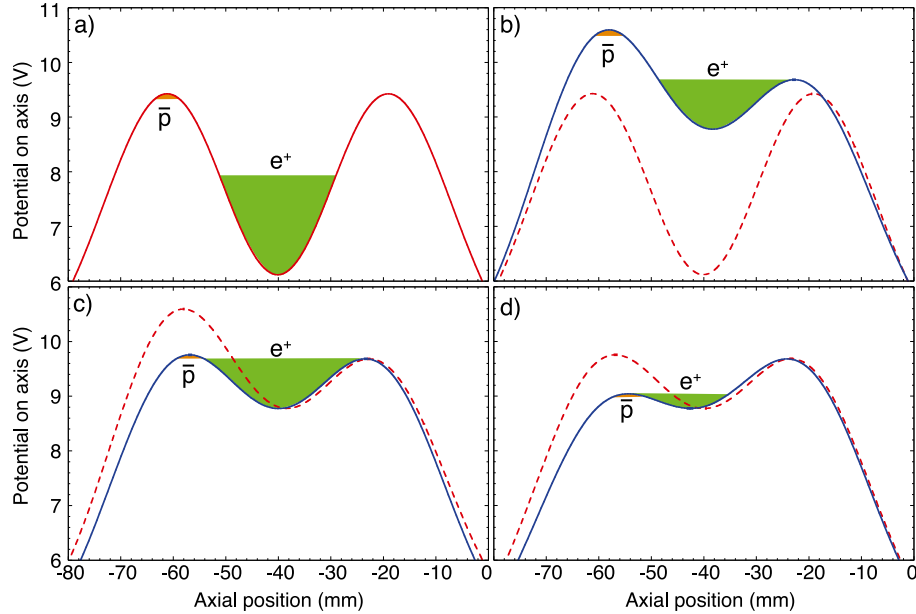
Fig. 15. Electrode potentials in the Atom Trap region when mixing positrons and antiprotons. The curves represent the electrostatic potential before (dashed) and after (solid) each step of the manipulation: (a) The potential before evaporative cooling; (b) evaporative cooling during which positrons escape to the right; (c) preparation for mixing (duration 10 ms); (d) Potential merge mixing (duration 1s). Positrons escape to the left during mixing, resulting in further evaporative cooling. After mixing is complete, any remaining positrons are ejected to the right while any remaining antiprotons are ejected to the left.
