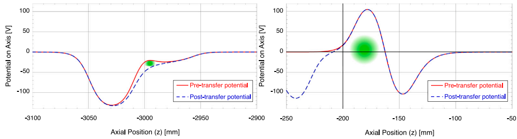
Fig. 14. Electric potentials on axis in the Catching (left) and re-catching (right) traps for the transfer of antiprotons. The axial positions are absolute relative to the centre of the Mixing Trap (A14). The re-catching trap potential change, effected by a fast gate, is applied at a delayed time relative to the change in the Catching Trap. Representative charged particle clouds (in green) indicate the nominal position of trapped antiprotons before (left) and after (right) the transfer.
