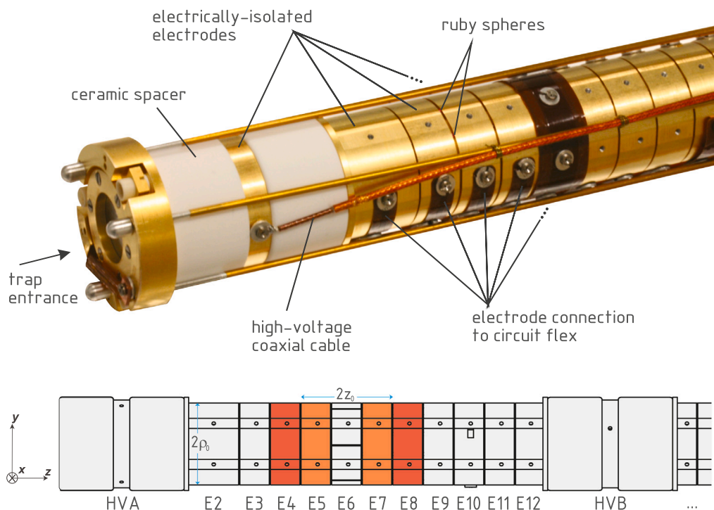
Fig. 5. A photograph (top) and schematic (bottom) of the Catching Trap electrodes. High voltage electrodes (HVA and HVB) are used for the initial antiproton capture; the remaining electrodes are used to manipulate antiproton and electron plasmas.
