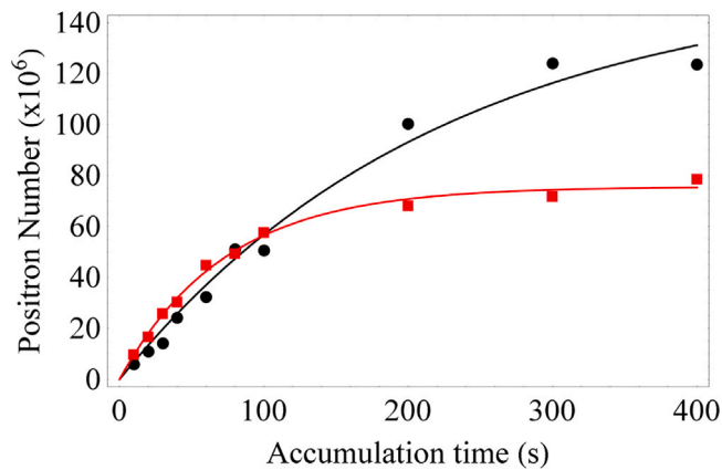
Fig. 11. Accumulated positron number N_e(t) versus accumulation time, t , for nitrogen pressures of 5 \times 10^{-4} mbar (black filled circle) and 1 \times 10^{-3} mbar (red filled square) in the first-stage. The solid lines are fits to the function N_e(t) = R\tau_e(1 - \exp(-t/\tau_e)) , where R is the accumulation rate and \tau_e is the positron lifetime within the apparatus. Accumulation rates of (7.0 \pm 0.6) \times 10^5 s ^{-1} and (1.04 \pm 0.04) \times 10^6 s ^{-1} , and lifetimes of (223 \pm 35) s and (73 \pm 4) s, are obtained at the lower and higher pressures respectively.
