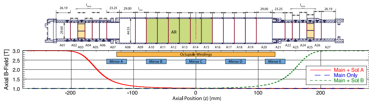
Fig. 12. Detail of the Mixing Trap electrodes. The ALPHA-2 Mixing Trap system consists of 27 cylindrical electrodes that can be individually biased. The Atom Trap is superposed on the central 13-electrode (A08 to A20) arrangement, and here the inner diameter is enlarged to 44.55 mm to enhance antihydrogen trapping. The inner diameter of the enclosing vacuum chamber is 48.00 mm. The two side traps have inner diameters of 29.60 mm and are used for preparing antiprotons (left side) and positrons (right side) for mixing. Two electrodes (A03 and A25 in yellow) are six-way azimuthally segmented for application of rotating wall drives, and 6 electrodes (A10–A15 in green) are excited by heavily filtered amplifiers to reduce electronic noise. The lower pane shows the axial magnetic field in this region.
