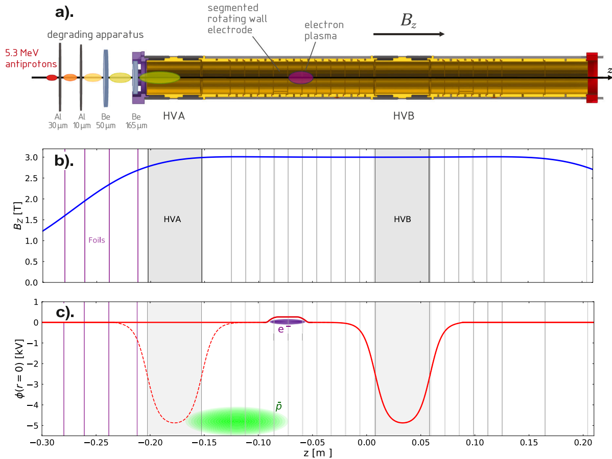
Fig. 6. (a) Rendering of the Catching Trap degraders and Penning trap. (b) Plot of the calculated axial magnetic field, B_z as a function of position. (c) The electric potential at the centre of the trap (at r = 0 ) before (solid line) and after (dotted line) antiproton capture, with representative charged particle clouds. This potential results from the application of discrete voltages to the electrodes.
