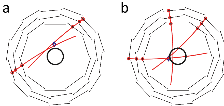
Fig. 25. The SVD reconstruction of (a) a typical cosmic ray event, and (b) a typical annihilation event. The red circles show the particle hit positions in the silicon modules, with the red lines the reconstructed tracks. The blue diamond indicates the inferred vertex position. The black inner ring marks the Atom Trap wall.
