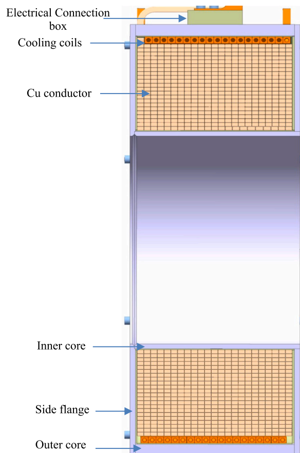
Fig. 18. Cross sections of the Catching to Atom Trap transfer magnets. The magnet produces a maximum field of B = 0.150 \text{ T} , and is used to transfer particles between sections of the ALPHA-2 apparatus. The coil is 140 mm long, with an inner aperture of 110 mm and an outer radius of 250 mm.
