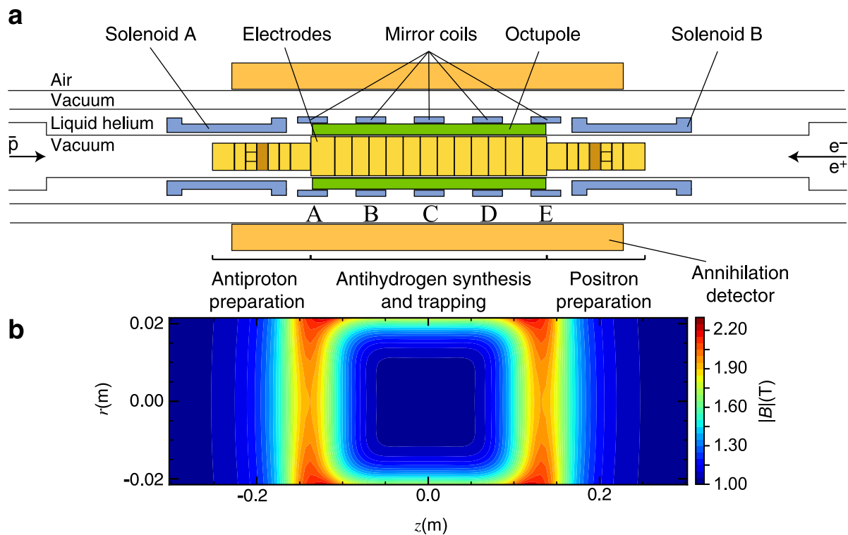
Fig. 16. (a) Schematic of the central portion of the Atom and Mixing Trap apparatus. The electrodes, together with a \sim 1 T background magnetic field, comprise the Mixing Trap which is used for charged particle manipulation. In the same physical location, the octupole and mirror coils comprise the Atom Trap, which forms a magnetic field capable of trapping a subset of the atoms that are created. (b) The magnetic field structure forms a minimum in |\vec{B}| . Atoms with energy equivalent less than about 0.5 K are confined in this field due to the interaction between their magnetic dipole moment and the magnetic field, which has potential energy U = -\vec{\mu} \cdot \vec{B} .
