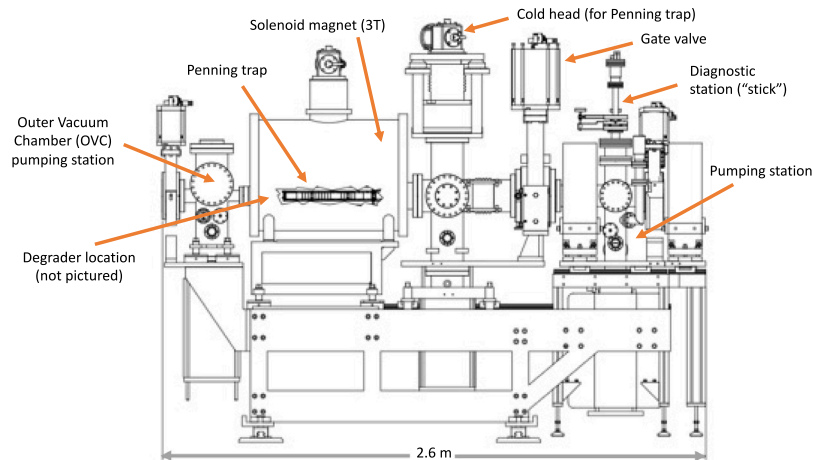
Fig. 2. Schematic of the Catching Trap and Transfer Magnet section of the ALPHA-2 apparatus. A cutaway shows the Penning-Malmberg trap inside the cryo-cooled magnet chamber. Not shown to the left of this diagram lies the evacuated beamline of the AD. Not shown to the right, an evacuated beamline connects to the Mixing and Atom Traps.
