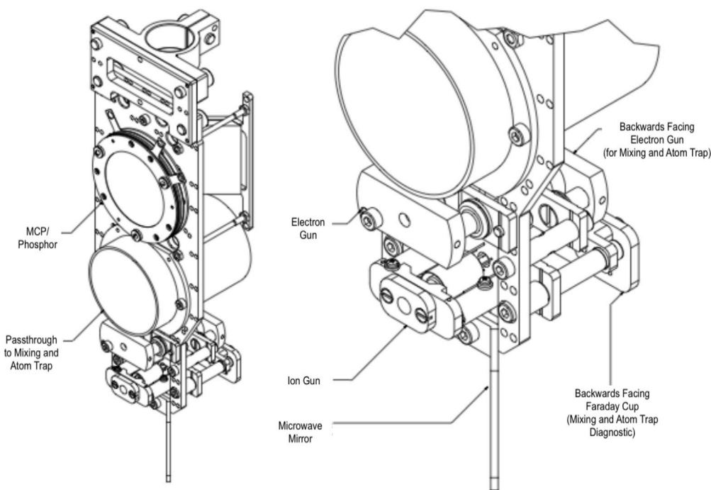
Fig. 8. Features of the Catching Trap diagnostic manipulator. The diagram on the left shows the full instrument panel. In the centre the MCP/Phosphor screen assembly and the grounded pass-through electrode are prominent. The right hand diagram features the electrode and the devices below it in more detail, including the forward- and backward-facing electron guns, the lithium ion source, an Atom Trap Faraday Cup diagnostic and a microwave mirror.
