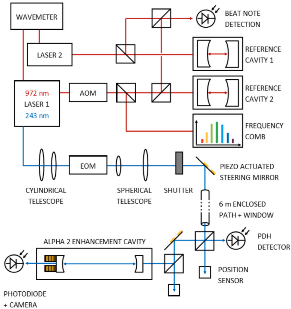
Fig. 20. Schematic of the 1S-2S laser system. A 972 nm external cavity diode laser (ECDL) is carefully measured and tuned, then frequency doubled twice. The resulting 243 nm light is delivered to the Mixing and Atom Trap, where the intensity is increased by the internal enhancement cavity.
