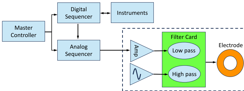
Fig. 7. Block diagram for the Catching Trap timing control. The master controller coordinates timing between digital and analog sequencers. The analog sequencer is primarily responsible for controlling the voltage on trap electrodes. The digital sequencer controls the timing of instruments such as diagnostics.
