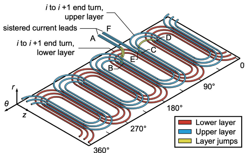
Fig. 17. Layout of the serpentine structure of the ALPHA-2 octupole coil. Note the cylindrical (r, \theta, z) coordinate system. See text for details.
