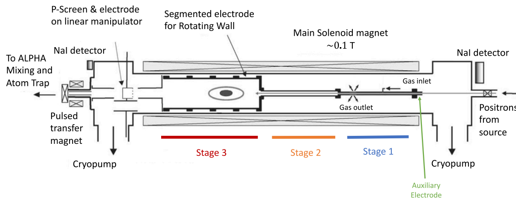
Fig. 10. Schematic illustration of the ALPHA-2 Positron Accumulator. Positrons enter from the beamline to the right and, once the accumulation cycle is complete, are ejected from the third, large diameter stage towards the main antihydrogen production and trapping region. A phosphor screen (viewed by an external camera, not shown) mounted on a linear manipulator can be used as a diagnostic of the transmitted positron beam and the ejected cloud.
