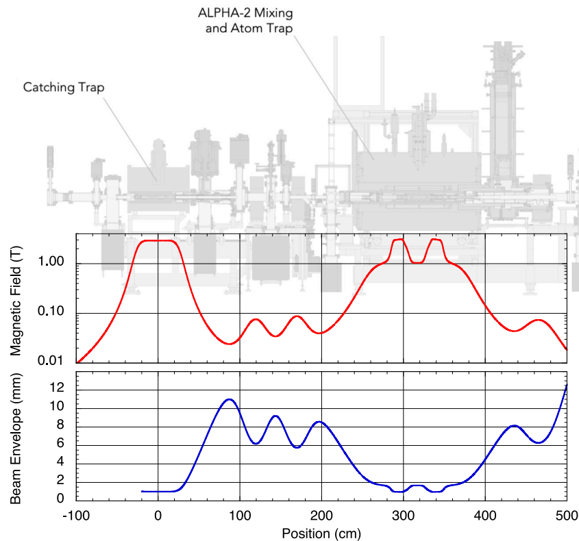
Fig. 19. Top: Plot of the calculated axial magnetic field ( B_z ) along the beam line and through the Atom Trap at the nominal operating points for the magnets. Bottom: Beam envelope for antiprotons with an initial radius of 1 mm extracted from the centre of the Catching Trap. A silhouette of the apparatus is superimposed for reference.
