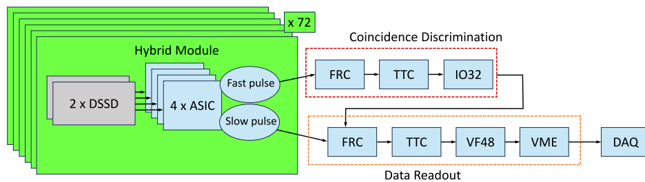
Fig. 24. Block diagram of the SVD readout system. Signals originate from particles depositing energy in the active area of the Silicon modules (DSSD). The signals are shaped by two independent integrated circuits on the same ASIC, which yield a fast and slow pulse. The former is compared to a fixed threshold, typically equivalent to 4800 electron-hole pairs, and the sum over the 128 channels is processed by an amplifier (FRC) and the timing module (TTC) for multiplicity trigger calculation. The final trigger decision is made by an FPGA (IO32) to determine whether the global multiplicity trigger condition is met. When this is the case, a readout trigger is sent to the FRC, prompting the sampling and multiplexing of the slow pulse data from the ASIC. While the analog readout has a fixed dead time of 40 \mu\text{s} (due to reading 128 strips serially with a 3.33 MHz clock), the limiting factor in the maximum event readout rate is due to the speed of the data transfer on the VME bus.
