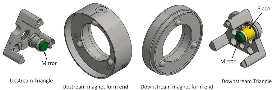
Fig. 21. From left to right: The upstream triangle, the upstream end of the magnet form, the downstream end of the magnet form, and the downstream triangle. Both triangles contain two slots for mounting a mirror assembly, but are shown with only one mirror assembly installed.
