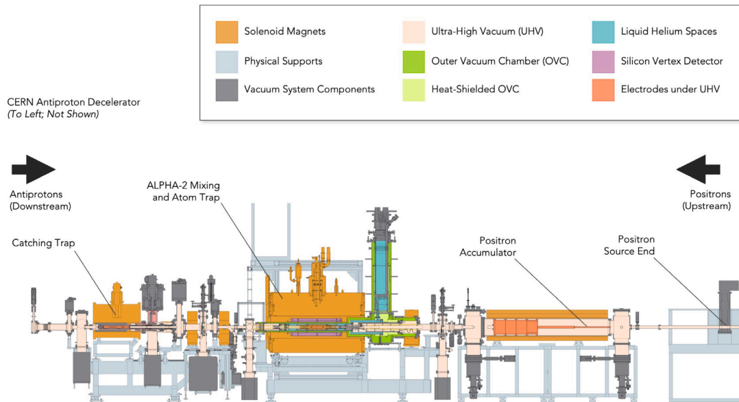
Fig. 1. An overview schematic of the ALPHA-2 apparatus in its 2017–19 configuration. The major sections of the ALPHA-2 apparatus include the Catching Trap (left), the Mixing and Atom Trap (centre), and the Positron Accumulator (right).
