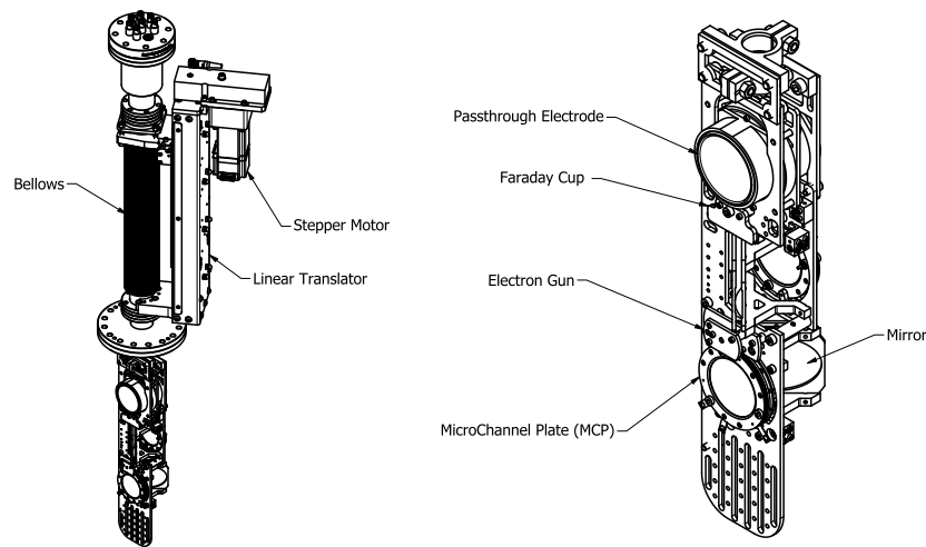
Fig. 13. Diagnostic manipulators for the Mixing Trap. Left: Rendering of the (internal) diagnostic array attached to the (external) linear translator via bellows. Right: A closer view of the diagnostic array which includes a passthrough electrode, an electron gun, an MCP, and a Faraday Cup plate. Another Faraday Cup, electron gun, and MCP are mounted on the back.
