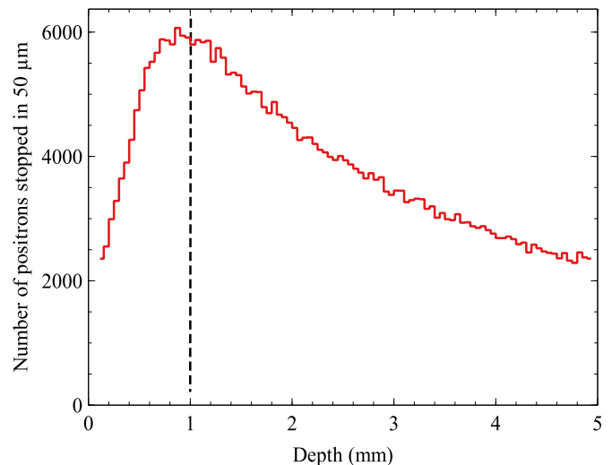
Fig. 2. Positrons created by 9 MeV electrons and stopped in a tungsten plate (GEANT4 simulation with 10^7 electrons). The number of positrons annihilating in 0.05 mm thick layers is plotted as a function of the depth. The dashed line at 1 mm shows the thickness of the actually used electron target.
