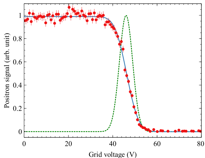
Fig. 7. Positron annihilation signal as a function of the voltage of the grid of the retarding field analyzer at 50 V moderator voltage. At low grid potential all positrons are annihilated on the target while above approximately 60 V all particles are repelled by the grid and no positron signal is detected. The continuous line is a fit with a complementary error function, giving \sigma_{\parallel} = 4.2 eV. The dotted line shows the corresponding Gaussian energy distribution. The measurement was performed in a 60 mT longitudinal magnetic field.
