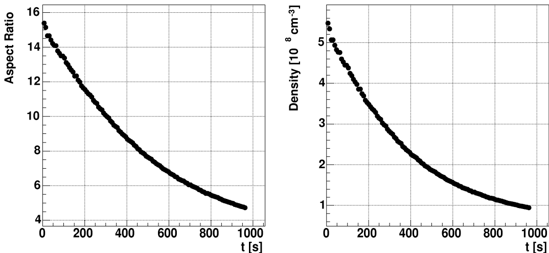
FIGURE 5. The evolution of the aspect ratio and the number density for a plasma of about 4 \times 10^7 positrons confined in the nested trap for about 1000 s without injection of any antiprotons.
