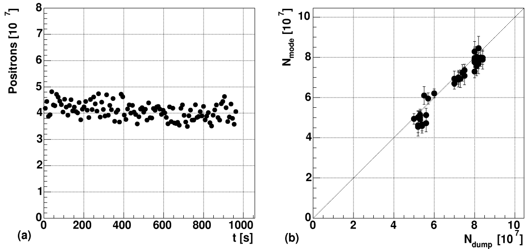
FIGURE 7. (a) Total number of positrons estimated by means of the transmission diagnostic for the plasma evolution of Fig. 5. (b) The total number of positrons obtained by using the transmission diagnostic is plotted against the number obtained by extracting the positrons to a Faraday cup.
