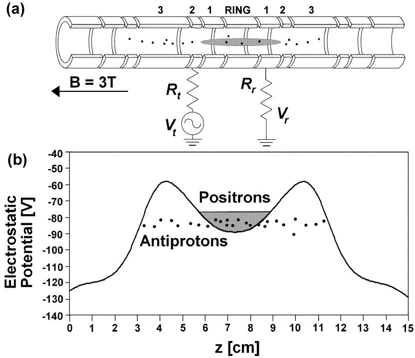
FIGURE 1. (a) Schematic of the mixing trap electrodes. The positrons are confined in the center group designed to create a harmonic electrostatic field. The central electrode is called the ring electrode and the other 3 pairs are labeled 1, 2 and 3. The driving signal applied to one electrode is shown together with the resistances on the transmitting and receiving electrodes. The shape of the prolate positron ellipsoid is shown schematically. (b) The axial potential of the ATHENA nested trap is shown and the ranges of axial motion of the positrons and of the antiprotons is indicated schematically.
