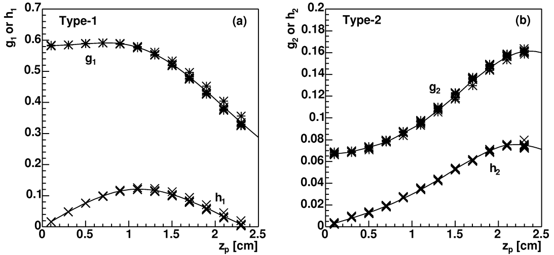
FIGURE 2. Dependence of the characteristic functions describing the coupling between the perturbation signal and dipole ( g_i ) and quadrupole ( h_i ) modes on the plasma semi-length for (a) type-1 and (b) type-2 electrodes (see the discussion in the text). The values are evaluated using the EQUILSOR-RATTLE numerical Poisson solver. The scattering of the points reflects the dependence on the aspect ratio. The solid curves are for aspect ratio \alpha = 6 .
