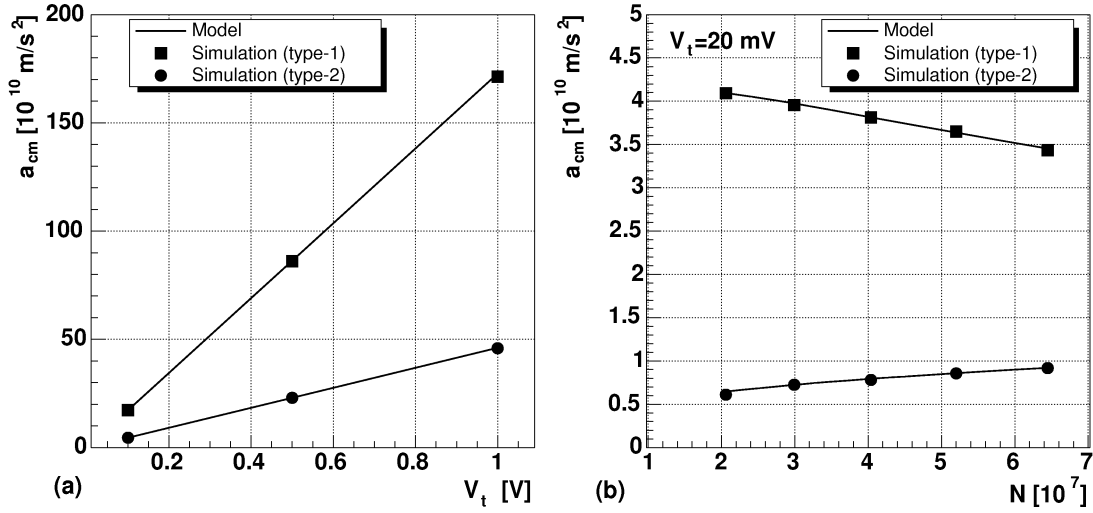
FIGURE 3. (a) Dependence of the acceleration amplitude a_{cm} of the center-of-mass oscillation on the amplitude of the perturbation V_t applied in resonance with \omega_1 . The time duration of the perturbation is limited to a few cycles of the dipole oscillation. Otherwise, for V_t > 0.1 V saturation effects are soon visible. The plasma was characterized by z_p = 1.63 cm, r_p = 0.22 cm, n = 2 \times 10^8 \text{ cm}^{-3} , and temperature T = 0.1 meV. (b) Acceleration amplitudes a_{cm} of the center-of-mass oscillation for different plasmas subjected to an external sinusoidal perturbation V_t \sin \omega_1 t applied on a type-1 or type-2 electrode. The simulated plasmas are characterized by different values of particle number N and axial semi-length z_p but they have all the same radius r_p = 0.22 cm. In both (a) and (b) the solid lines are the growth rates evaluated according Eq. (5).
