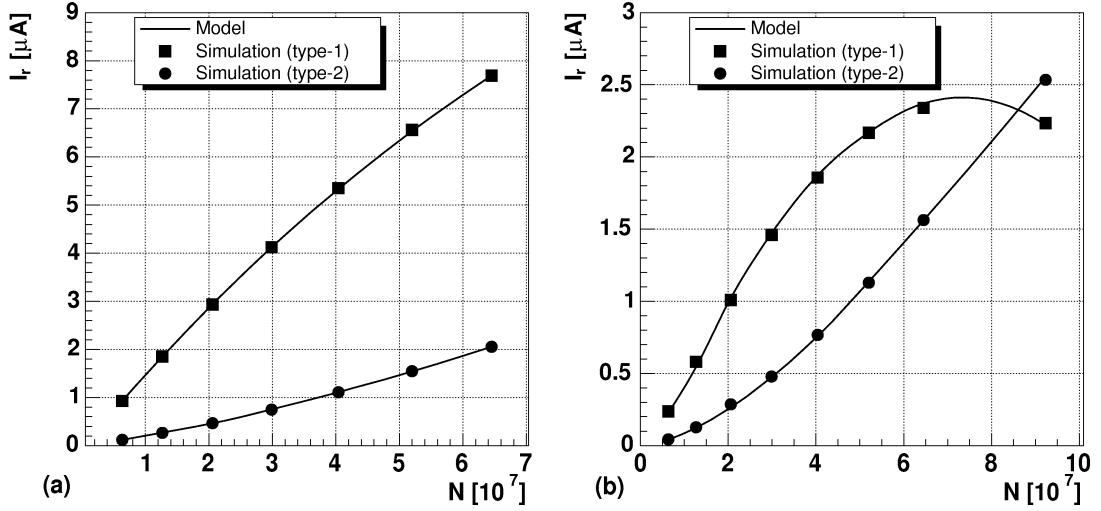
FIGURE 4. (a) Simulated induced current on the trap electrodes due to the oscillation of the center-of-mass for different plasmas ( z_{\text{offset}} \simeq 0.3 mm). The solid lines represent the values of the induced currents evaluated by means of Eq. (7). (b) Simulated induced current on the trap electrodes due to the quadrupole mode for different plasmas ( z_{\text{stretch}} \simeq 0.3 mm). The solid lines represent the values of the induced currents evaluated by means of Eq. (10).
