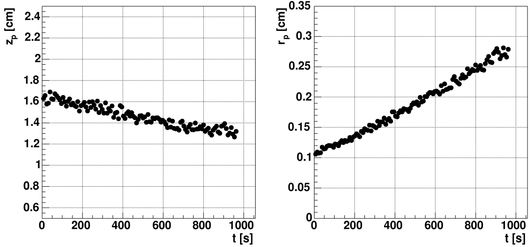
FIGURE 6. The evolution of the plasma semi-length and radius for the plasma as Fig. 5.
