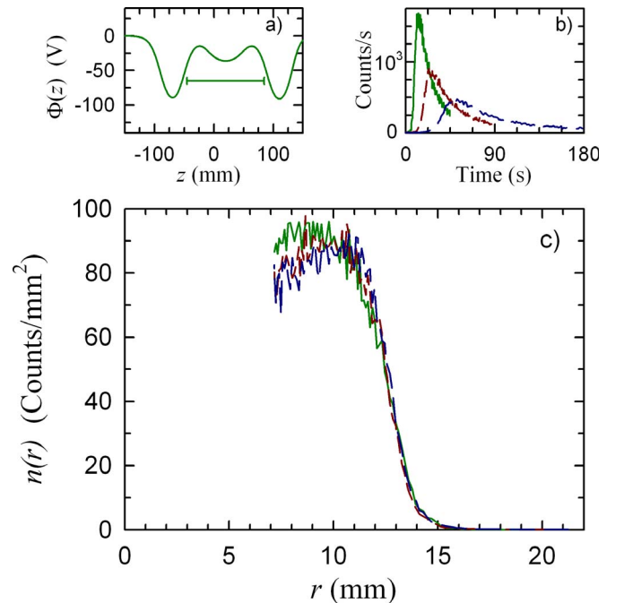
FIG. 8. (Color online) Comparison of the radial profiles with octupole ramps of 45 (green solid), 90 (red short-dash), and 180 s (blue long-dash). The well length in each case was 130 \pm 5 mm. The graph descriptions and all other parameters are the same as in Fig. 6.
