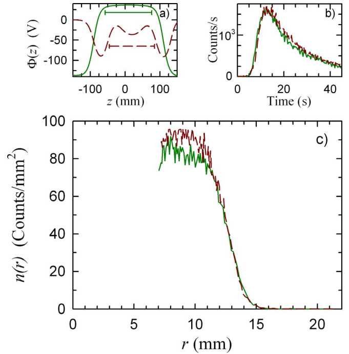
FIG. 7. (Color online) Comparison of the radial profiles obtained with flat (green solid) and nested well potentials (red dash). The well lengths were 135 \pm 5 and 130 \pm 5 mm, respectively. The graph descriptions and all other parameters are the same as in Fig. 6.
