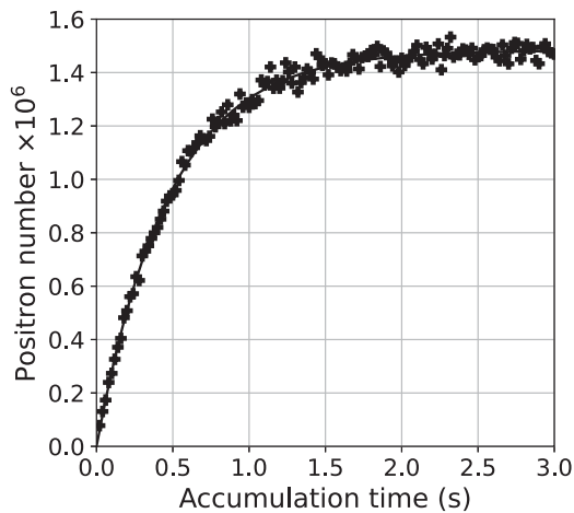
Fig. 7. Positron accumulation in the second stage. RW parameters: 2 MHz, 1 V. Fitting the measured values to Eq. (6) yielded \tau = 0.470(1) s and R = 3.10(6) \times 10^6 \text{ s}^{-1} .
