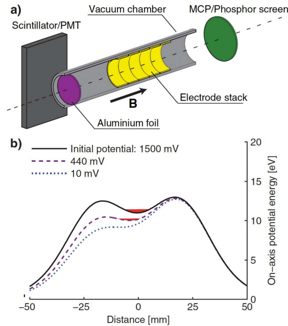
Figure 4. (a) Simplified schematic of the Penning-Malmberg trap used to confine the antiprotons and of the two diagnostic devices used. The direction of the magnetic field is indicated by the arrow. (b) Potential wells used to confine the antiprotons during the evaporative cooling ramp. The antiprotons are indicated at the bottom of the potential well (red), and the different wells are labelled by their on-axis depth.
