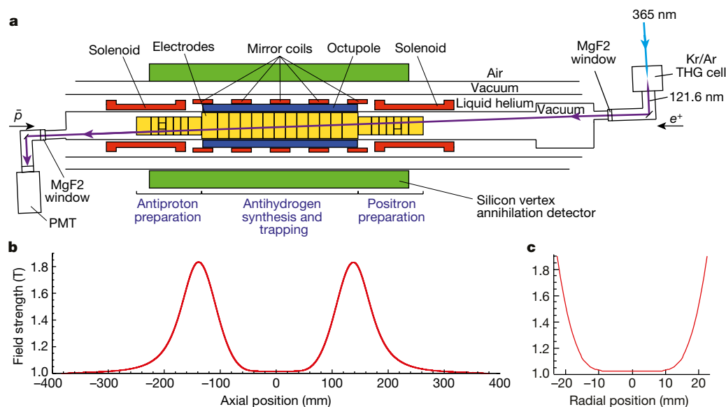
Fig. 1 | Experimental set-up. a , The three-layer silicon vertex annihilator detector is shown schematically in green; the external solenoid magnet for the Penning trap is not shown in this diagram. Laser light enters from the positron ( e^+ ) side (right) and is transmitted to the antiproton ( \bar{p} ) side (left) through vacuum-ultraviolet-grade MgF 2 ultrahigh-vacuum windows. The laser beam crosses the trap axis at an angle of 2.3°. The transmitted 121.6-nm pulses are detected by a photomultiplier at the antiproton side. b , Axial magnetic well formed by the five mirror coils and responsible for the axial confinement of cold (less than 0.5 K) anti-atoms. c , Radial magnetic octupole field profile. PMT, photomultiplier tube; THG, third-harmonic generation.
